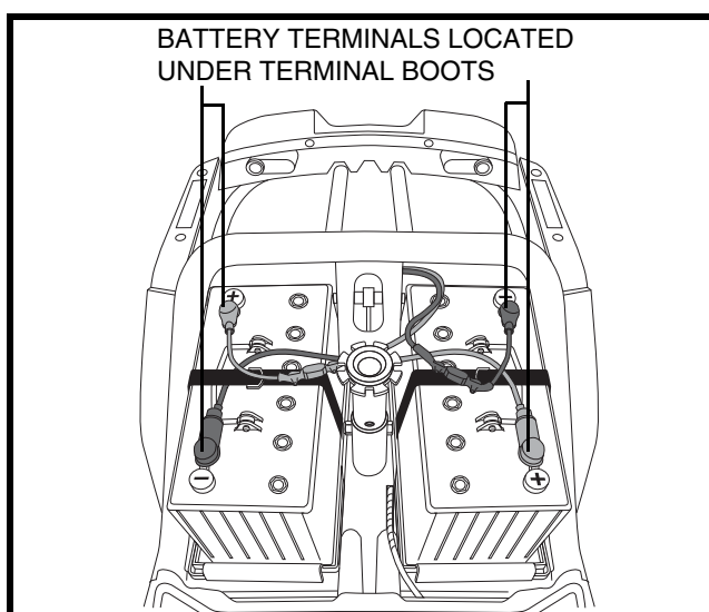
Figure 14. Battery Removal/Replacement
