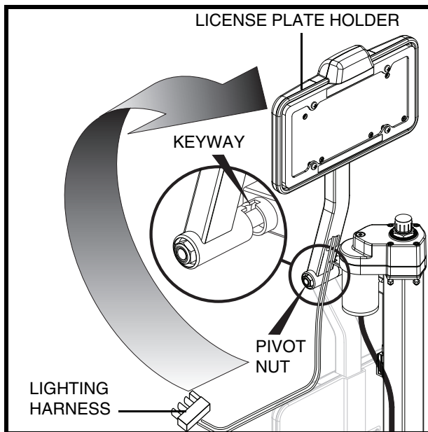
Figure 8. License Plate Holder
