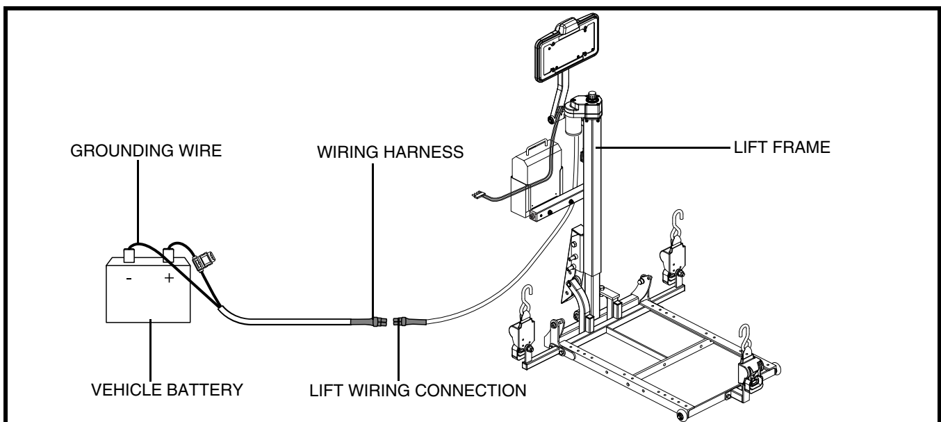
Figure 7. Wiring Harness Installation
