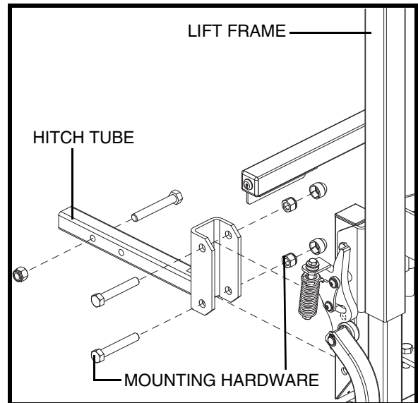
Figure 5. Hitch Tube Assembly
