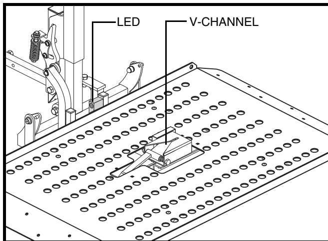
Figure 16. Power Dock
