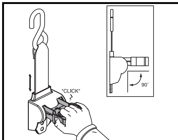
Figure 13. Unlocking the Retractable Tie-down Strap
