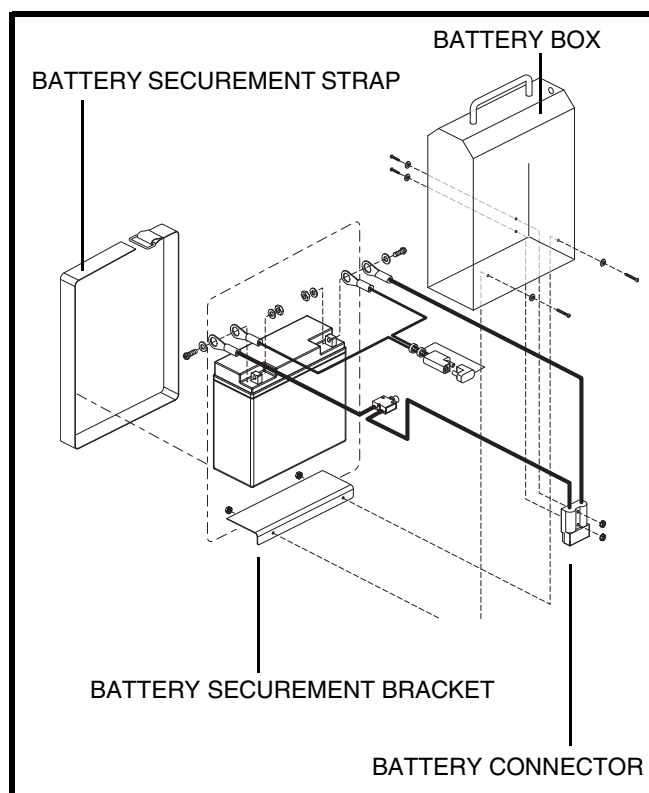
Figure 20. Battery Replacement
