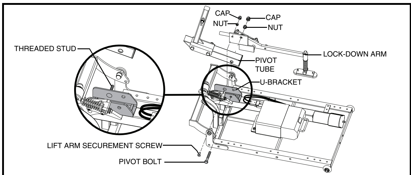
Figure 4. Lock-down Arm Installation
