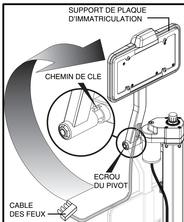
Figure 8. Support de plaque d'immatriculation
