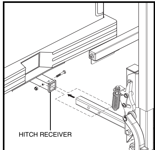
Figure 6. Lift Frame Vehicle Mounting
