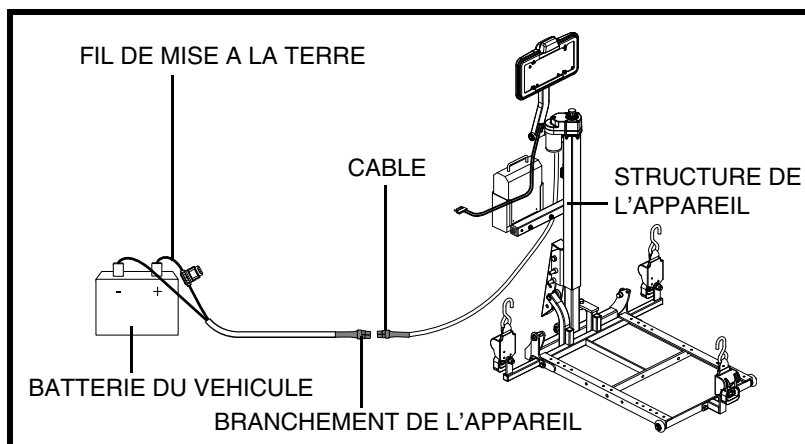
Figure 7. Installation du câblage
