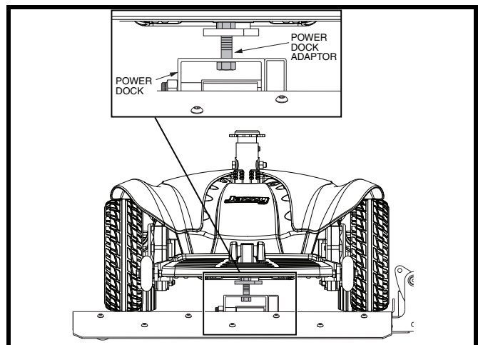
Figure 17. Power Chair Loaded
