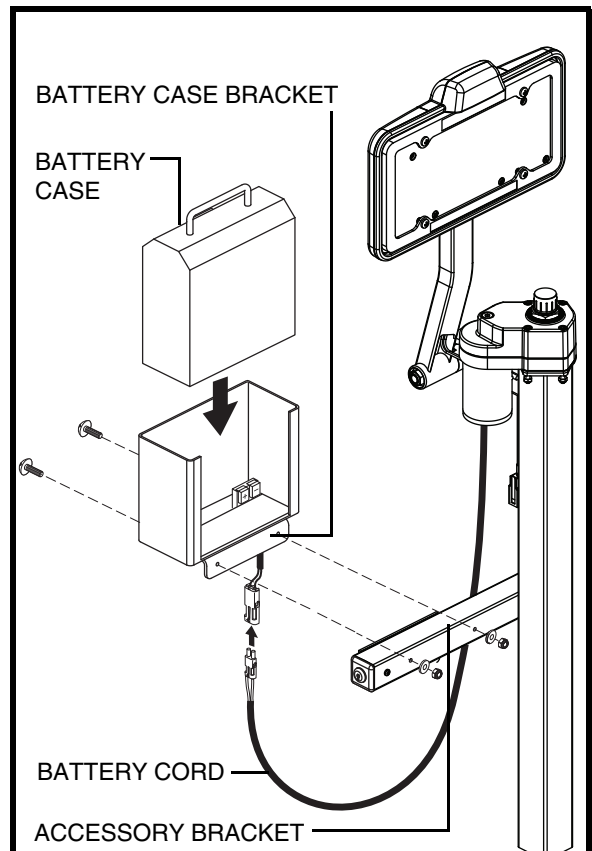
Figure 9. Onboard Battery Installation
