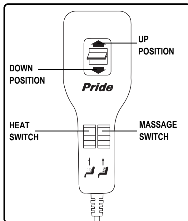
Figure 5.6 C40 Heat and Massage Hand Control
