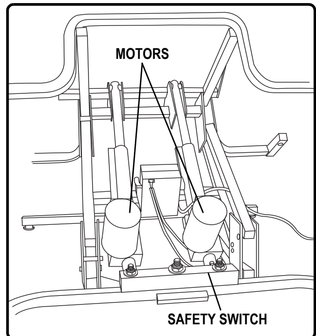
Figure 6.3 In-sync Motors (Timing Corrected)
