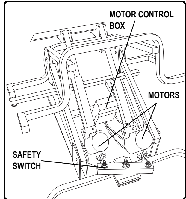
Figure 6.1 Out-of-sync Motors
