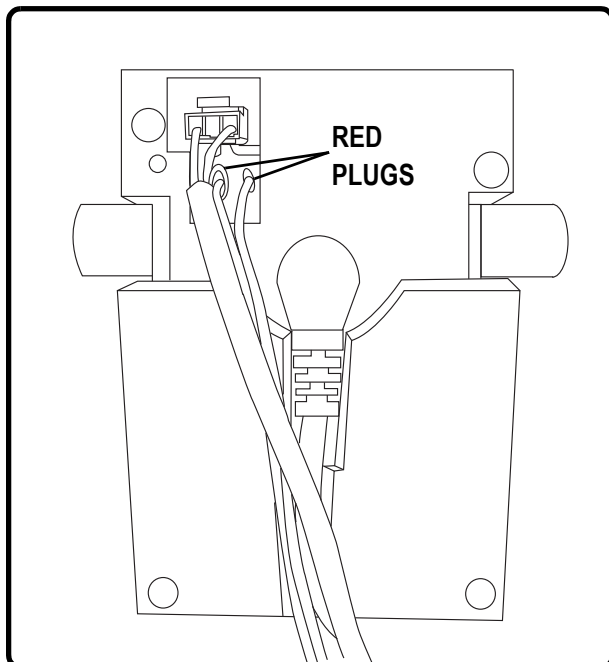
Figure 6.2 Safety Switch Plugs
