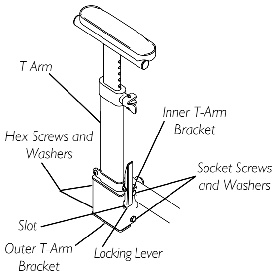
FIGURE 6 - ADJUSTING T-ARM SOCKETS
