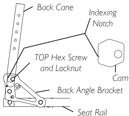
FIGURE I - BACK ANGLE ADJUSTMENT
