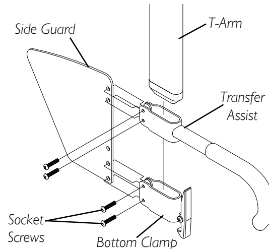
FIGURE 7 - ADJUSTING T-ARM TRANSFER ASSISTS AND/OR SIDE GUARDS
