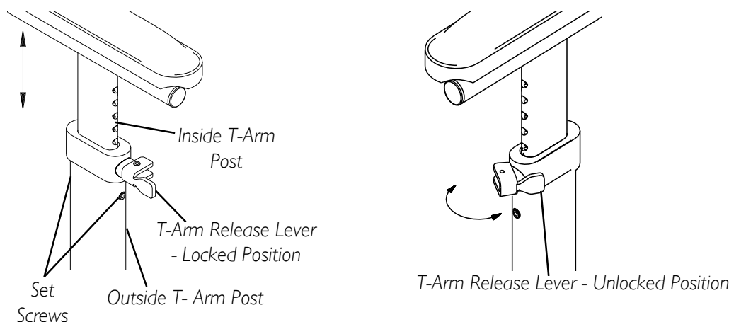
FIGURE 3 - ADJUSTING T-ARM HEIGHT
