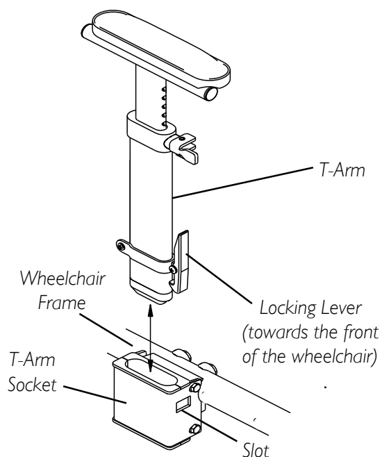
FIGURE 2 - INSTALLING/ REMOVING T- ARMS
