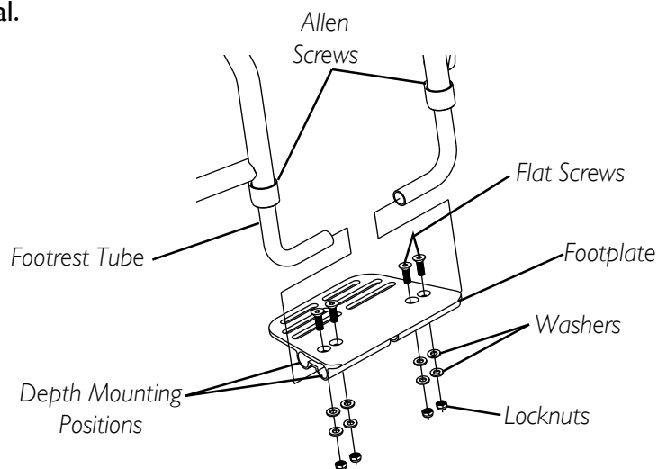
FIGURE 1 - FOOTREST REPLACEMENT/ADJUSTMENT
