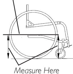
FIGURE 6 - DETERMINING TOE IN/TOE OUT
