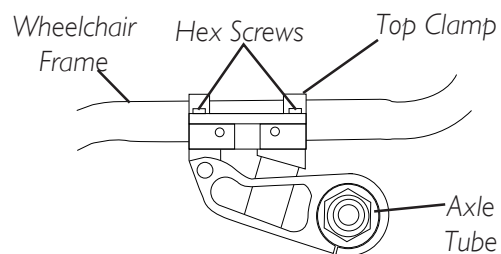
FIGURE 10 - ADJUSTING WHEELBASE LENGTH (ADJUSTING CENTER OF GRAVITY)
