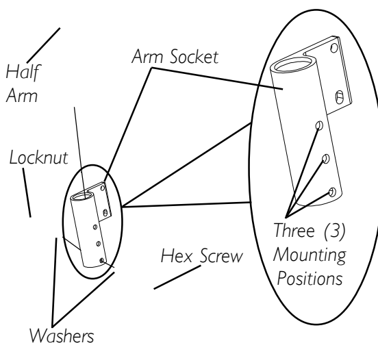
FIGURE 10 - ADJUSTING HALF ARM HEIGHT
