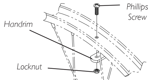
FIGURE 6 - HANDRIM REPLACEMENT
