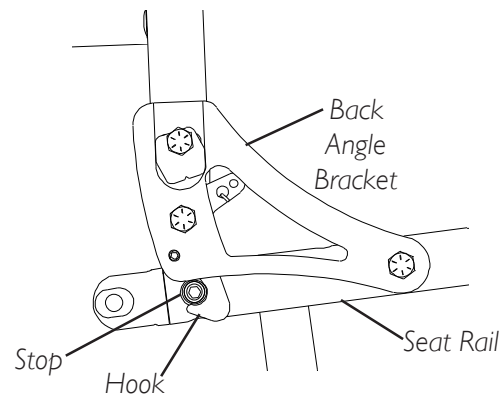
FIGURE 4 - REPLACING SEAT FRAME
