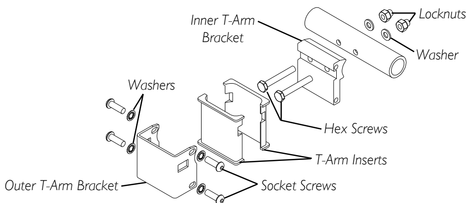
FIGURE 1 - INSTALLING THE T-ARM SOCKETS
