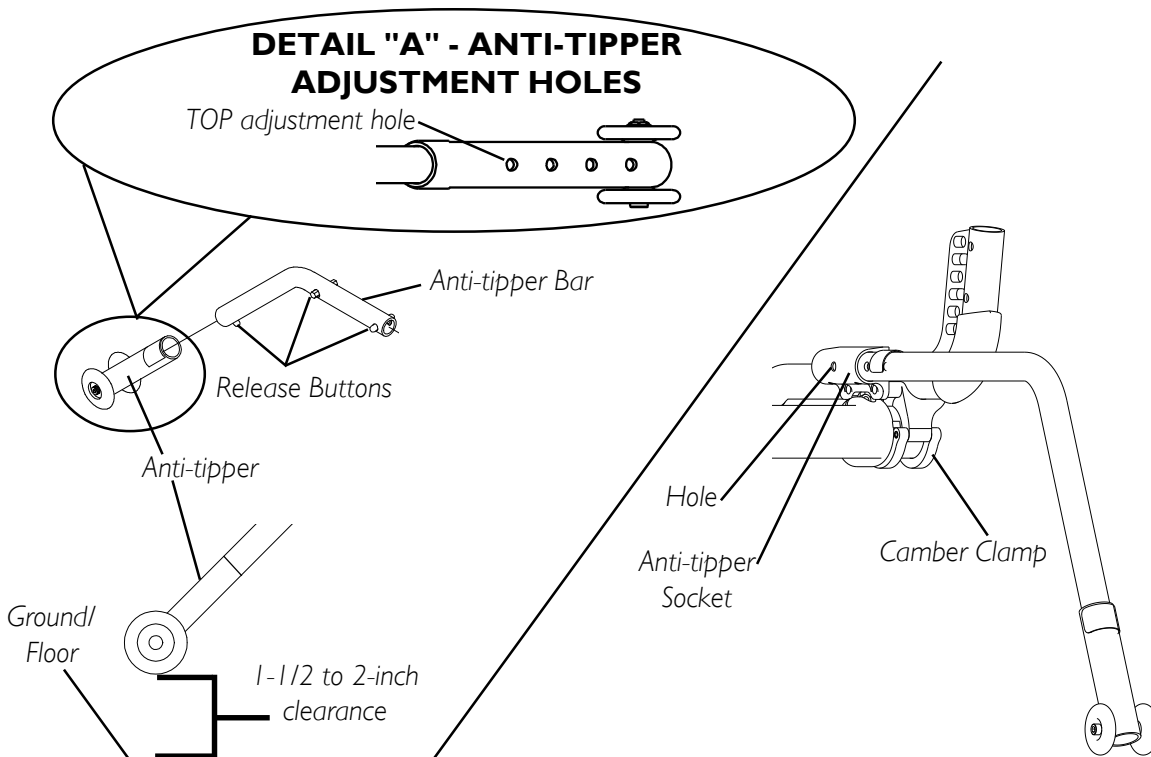
FIGURE 1 - ANTI-TIPPER ADJUSTMENT/REPLACEMENT
