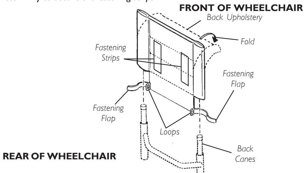
FIGURE 2 - REMOVING/INSTALLING STANDARD BACK UPHOLSTERY
